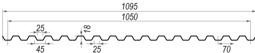
Profile GRECA 70x18
