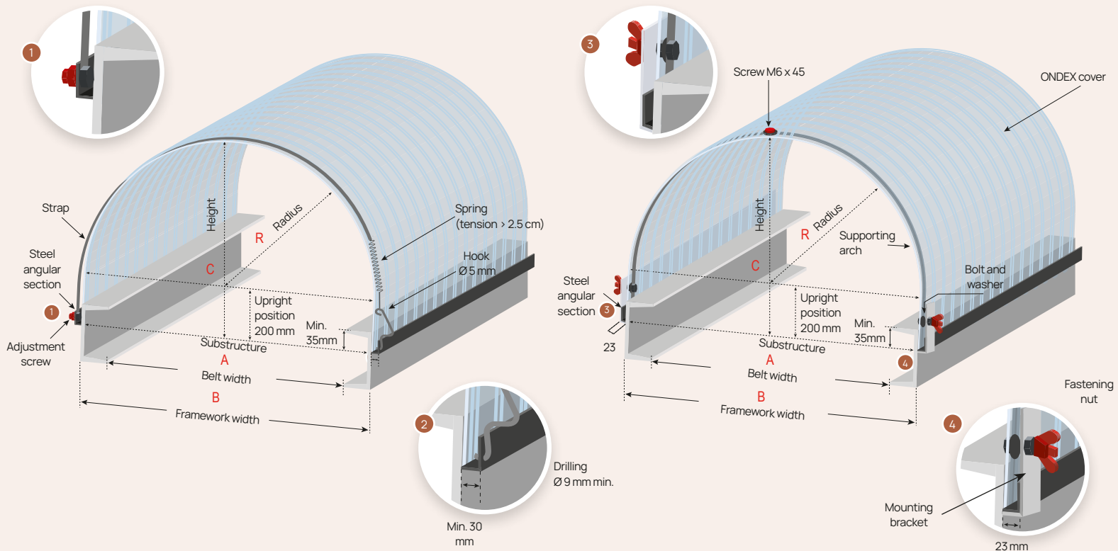
Fastening with strap for covers No. 1-2-3-4
